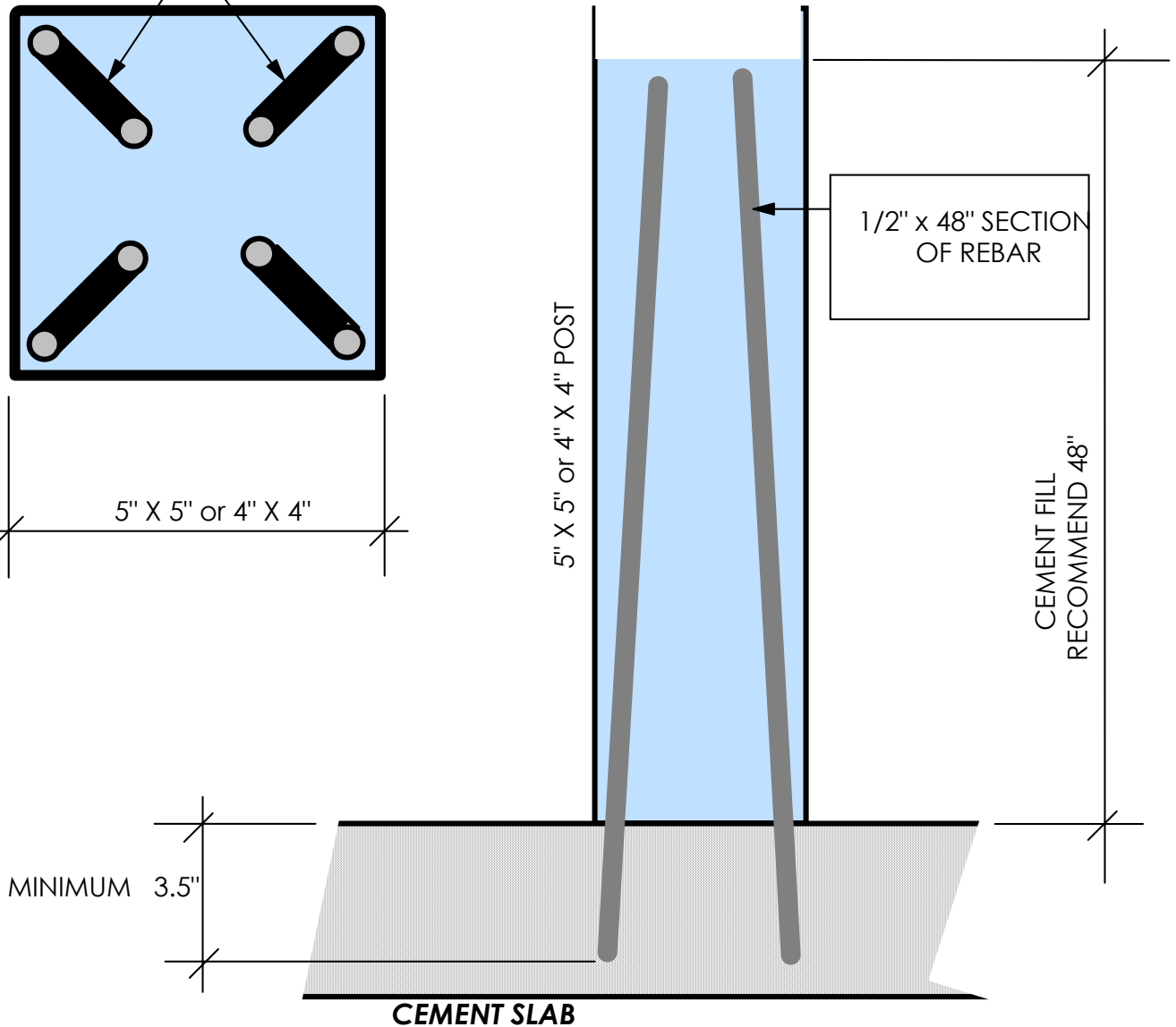
SIDE VIEW OF POST
